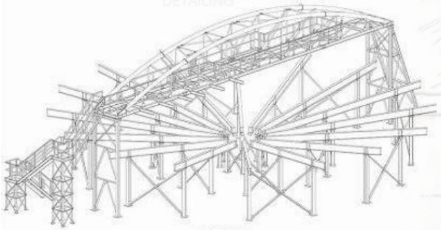
ISOMETRIC VIEW
